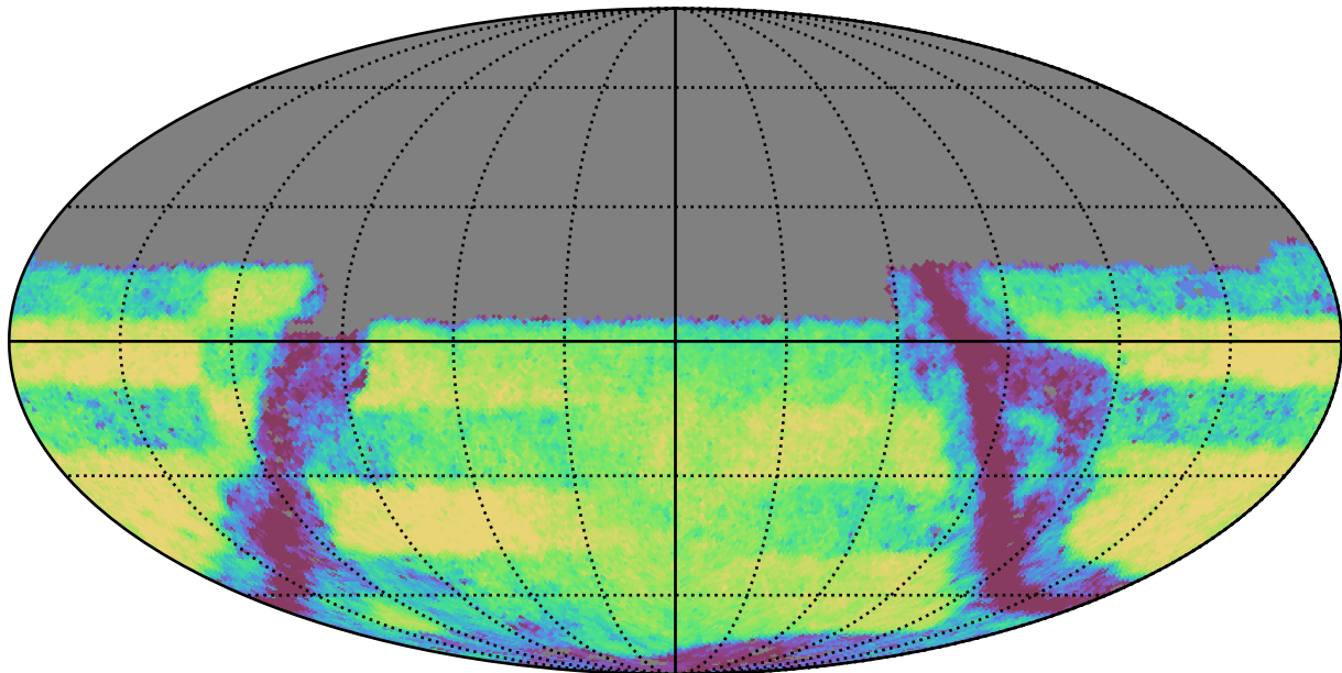
weather_cloudso18v3.4_10yrs Yr 3-4 y band: Exgal_CoaddM5
