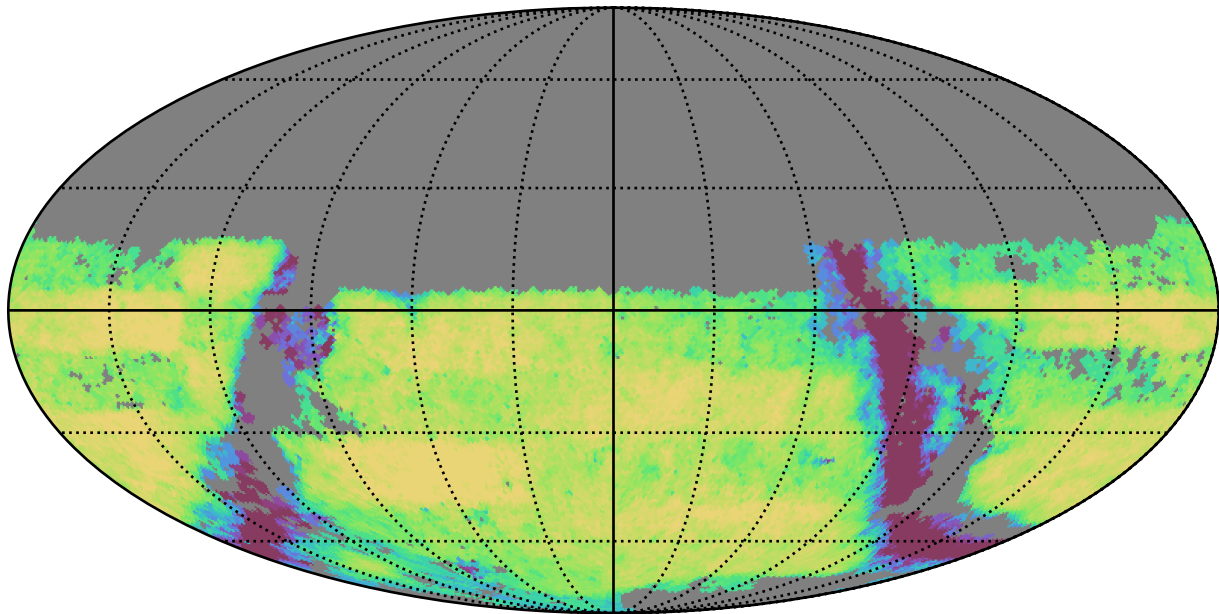
weather_cloudso18v3.4_10yrs Yr 3-4 u band: Exgal_CoaddM5
