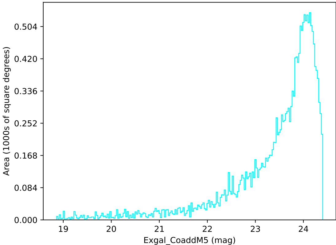
weather_cloudso18v3.4_10yrs Yr 3-4 u band: Exgal_CoaddM5
