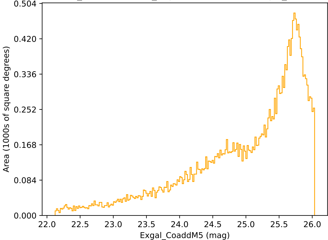
weather_cloudso18v3.4_10yrs Yr 3-4 r band: Exgal_CoaddM5
