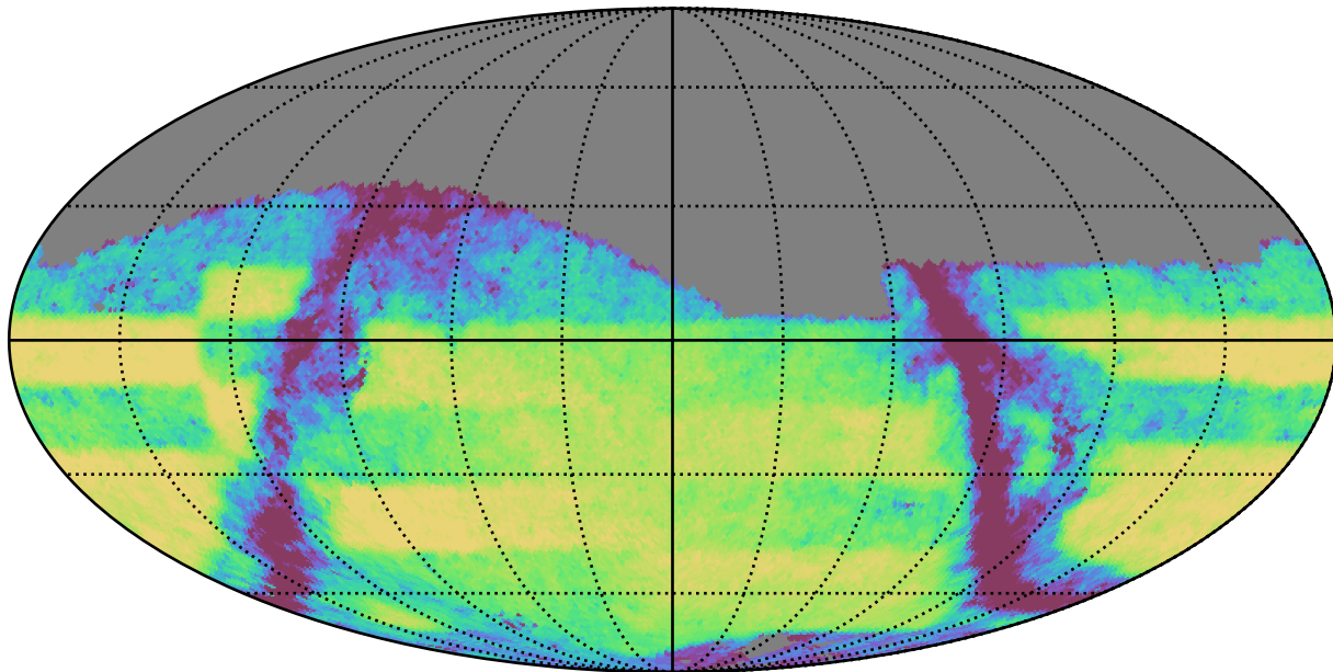
weather_cloudso18v3.4_10yrs Yr 3-4 i band: Exgal_CoaddM5
