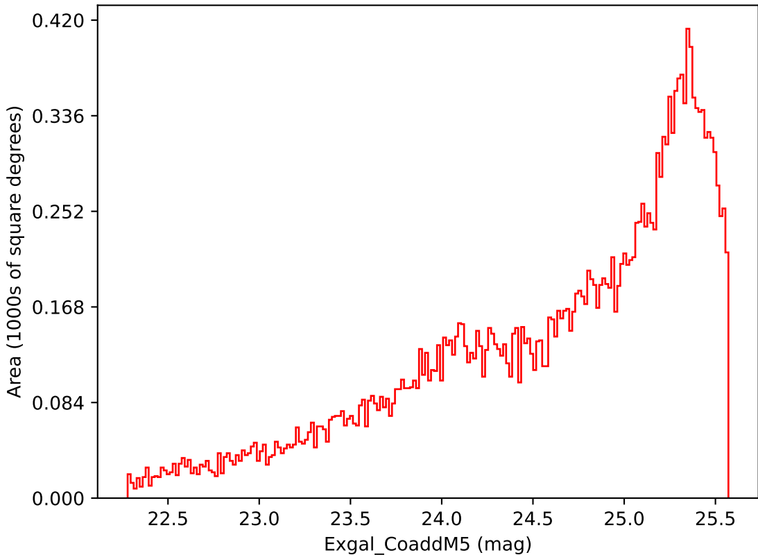
weather_cloudso18v3.4_10yrs Yr 3-4 i band: Exgal_CoaddM5
