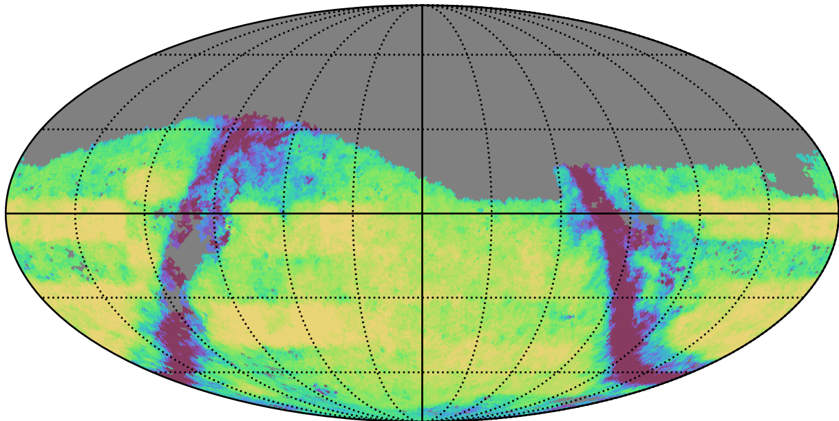
weather_cloudso18v3.4_10yrs Yr 3-4 g band: Exgal_CoaddM5
