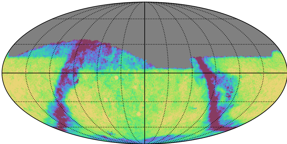
weather_cloudso18v3.4_10yrs Yr 1 z band: Exgal_CoaddM5
