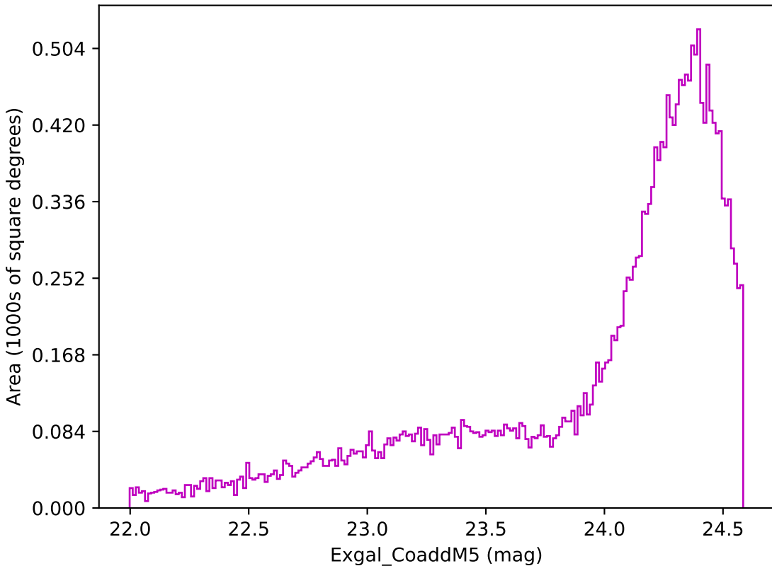
weather_cloudso18v3.4_10yrs Yr 1 z band: Exgal_CoaddM5
