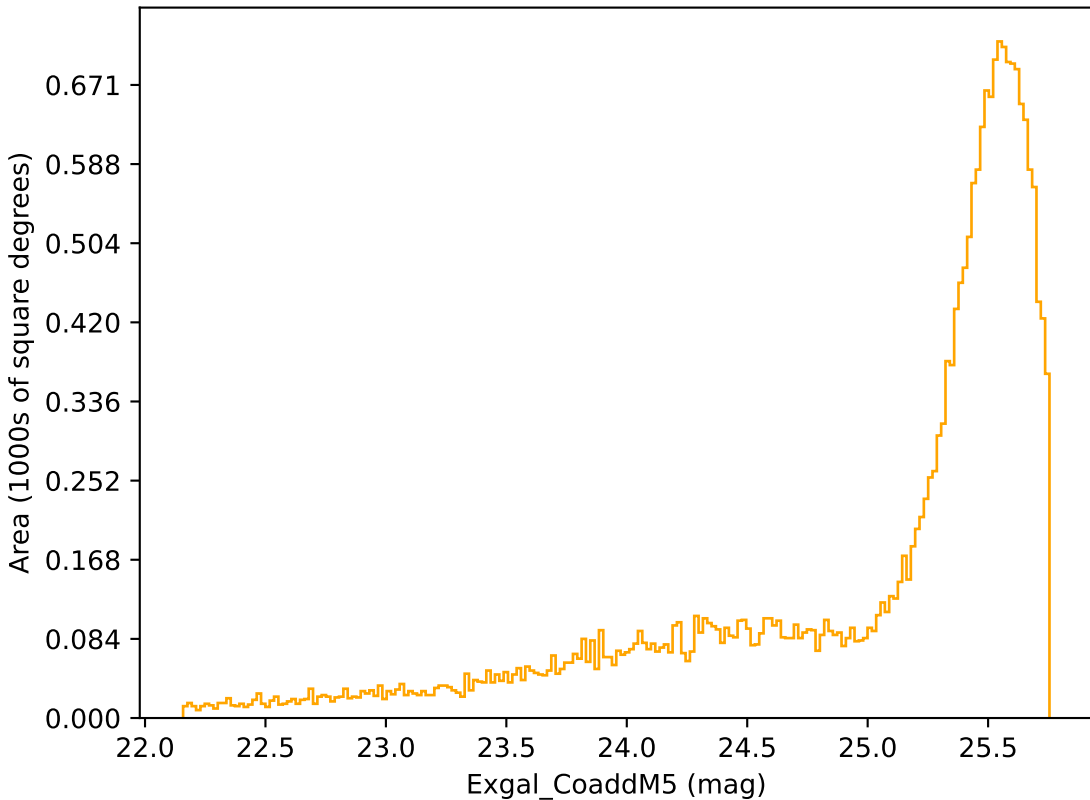
weather_cloudso18v3.4_10yrs Yr 1 r band: Exgal_CoaddM5
