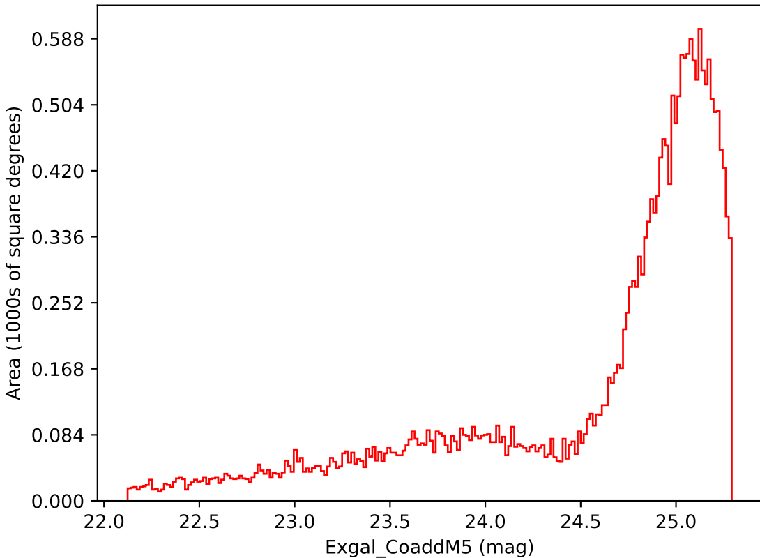
weather_cloudso18v3.4_10yrs Yr 1 i band: Exgal_CoaddM5
