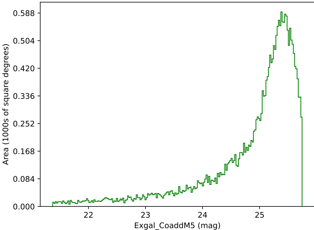
weather_cloudso18v3.4_10yrs Yr 1 g band: Exgal_CoaddM5
