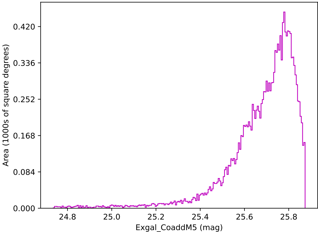
weather_cloudso18v3.4_10yrs WFD z band: Exgal_CoaddM5
