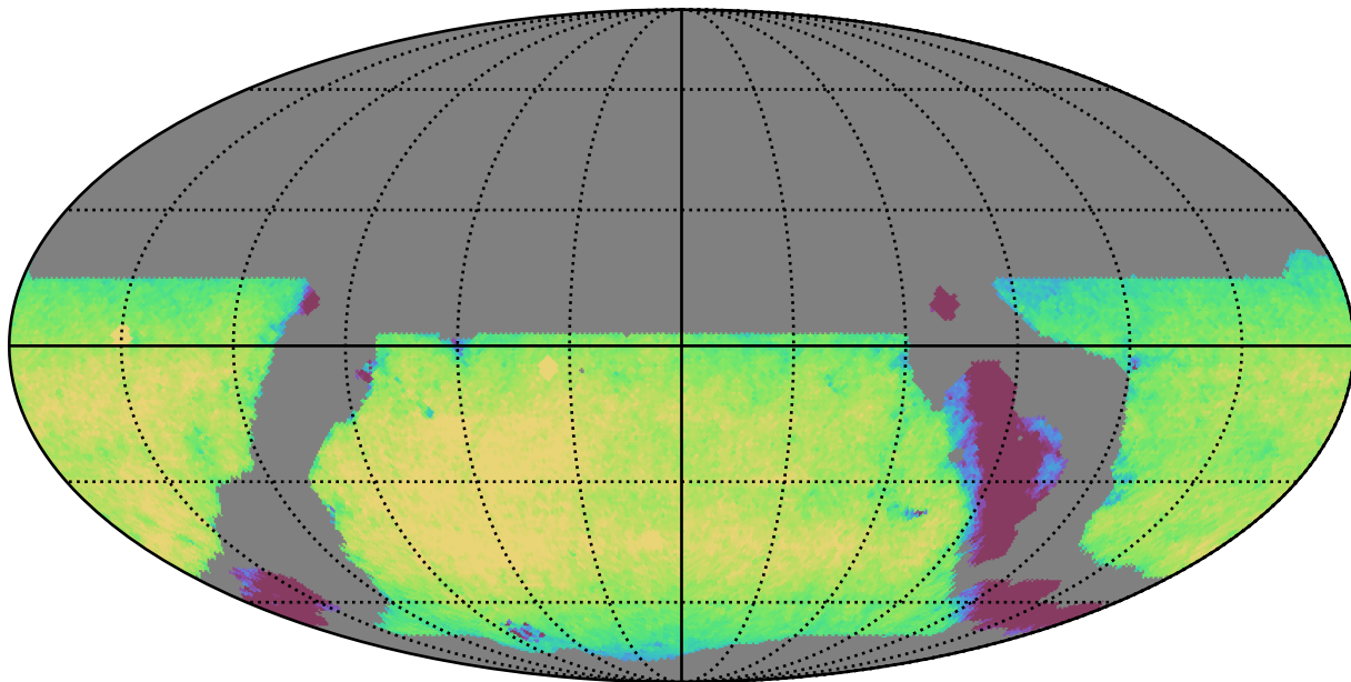
weather_cloudso18v3.4_10yrs WFD y band: Exgal_CoaddM5
