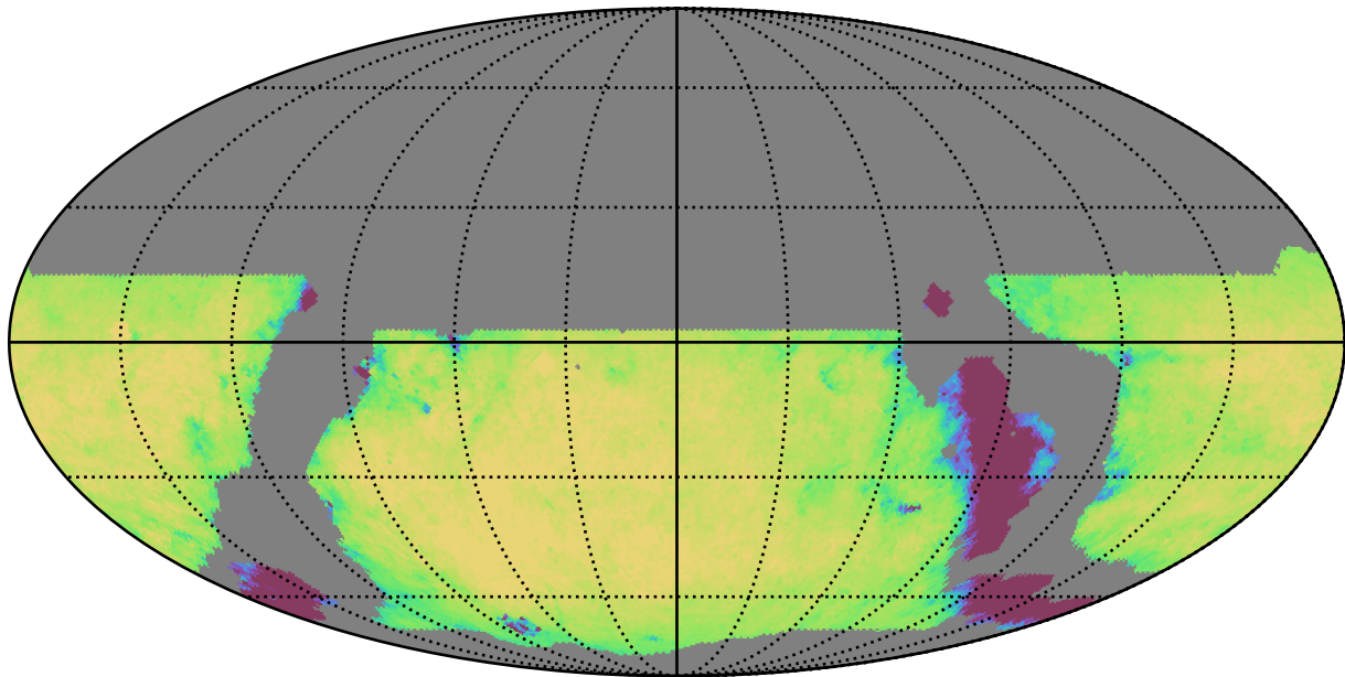
weather_cloudso18v3.4_10yrs WFD u band: Exgal_CoaddM5
