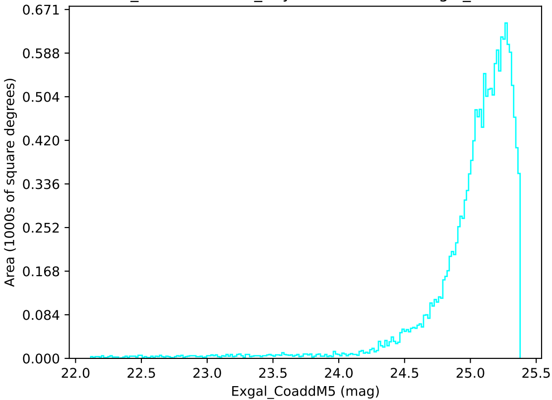
weather_cloudso18v3.4_10yrs WFD u band: Exgal_CoaddM5
