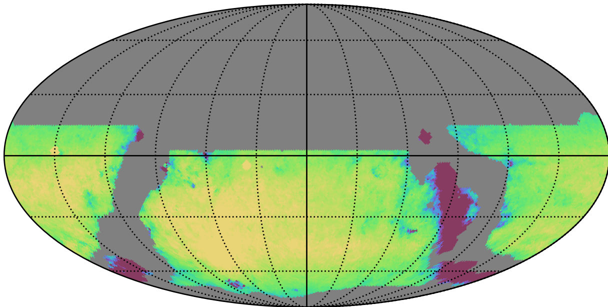
weather_cloudso18v3.4_10yrs WFD r band: Exgal_CoaddM5
