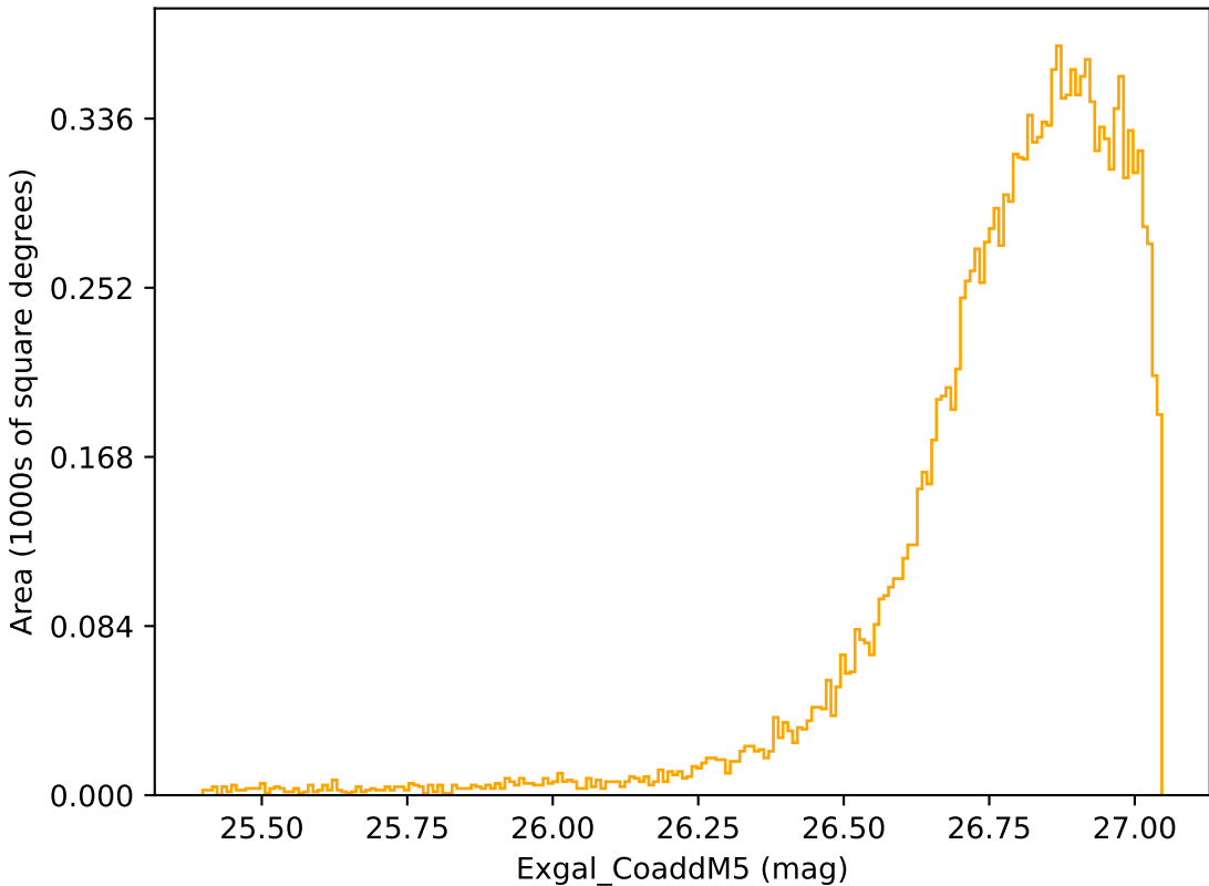
weather_cloudso18v3.4_10yrs WFD r band: Exgal_CoaddM5
