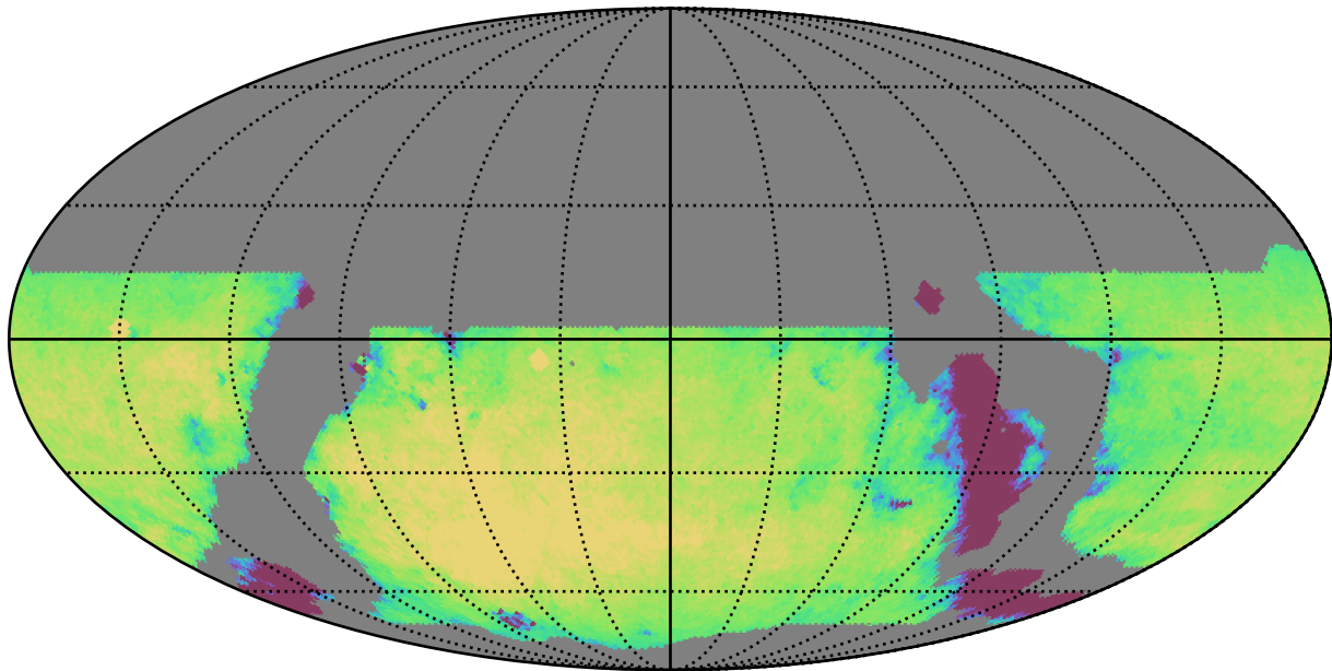
weather_cloudso18v3.4_10yrs WFD g band: Exgal_CoaddM5
