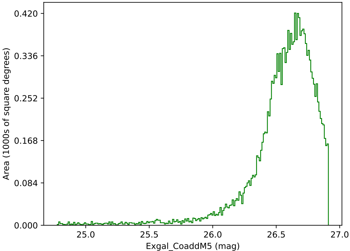
weather_cloudso18v3.4_10yrs WFD g band: Exgal_CoaddM5
