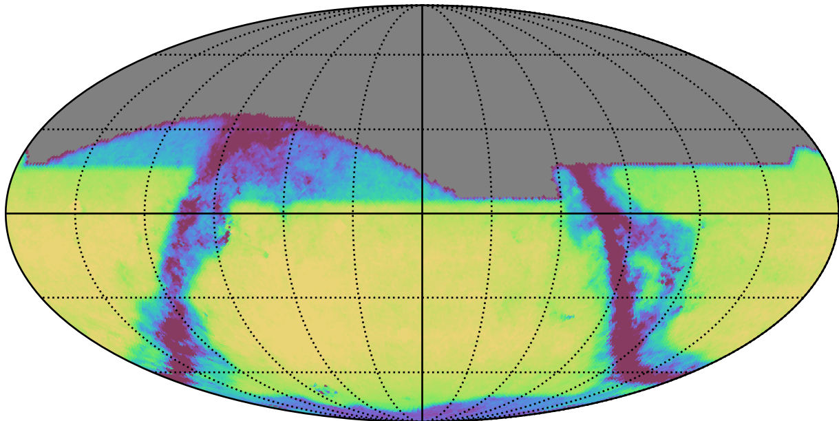
weather_cloudso18v3.4_10yrs All sky z band: Exgal_CoaddM5
