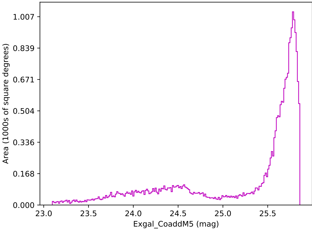
weather_cloudso18v3.4_10yrs All sky z band: Exgal_CoaddM5
