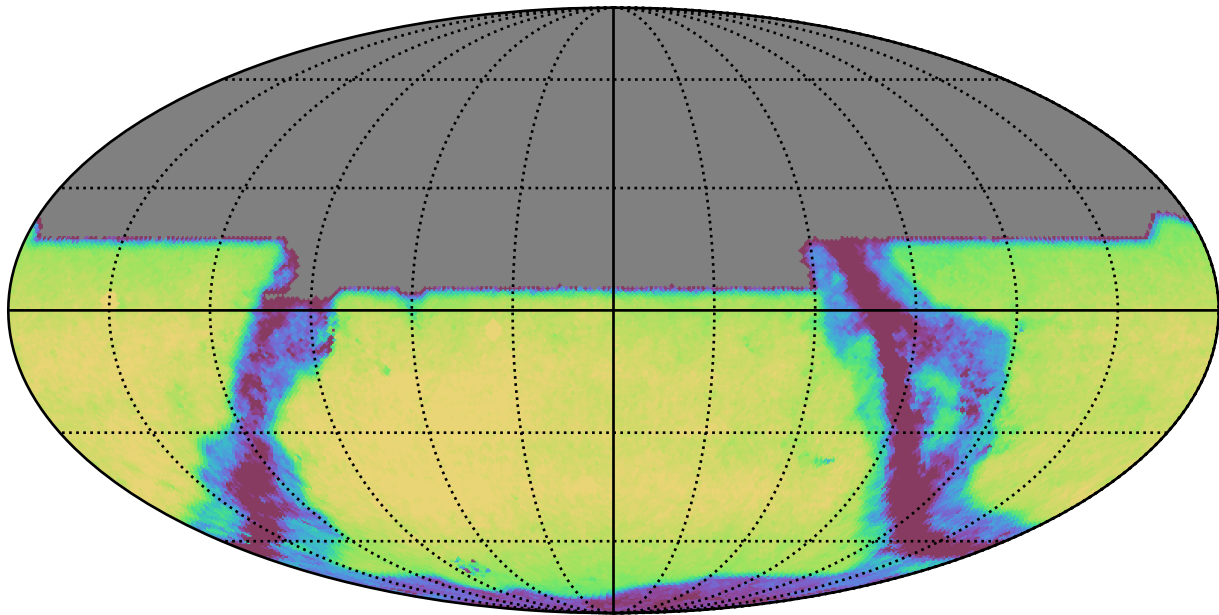
weather_cloudso18v3.4_10yrs All sky y band: Exgal_CoaddM5
