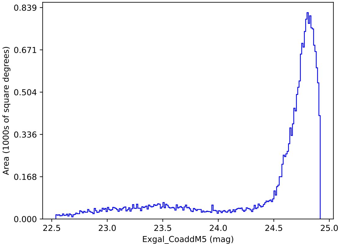
weather_cloudso18v3.4_10yrs All sky y band: Exgal_CoaddM5
