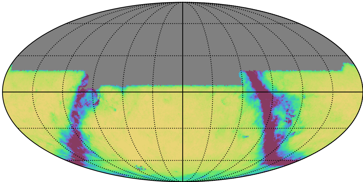
weather_cloudso18v3.4_10yrs All sky u band: Exgal_CoaddM5
