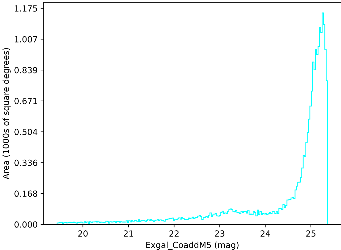
weather_cloudso18v3.4_10yrs All sky u band: Exgal_CoaddM5
