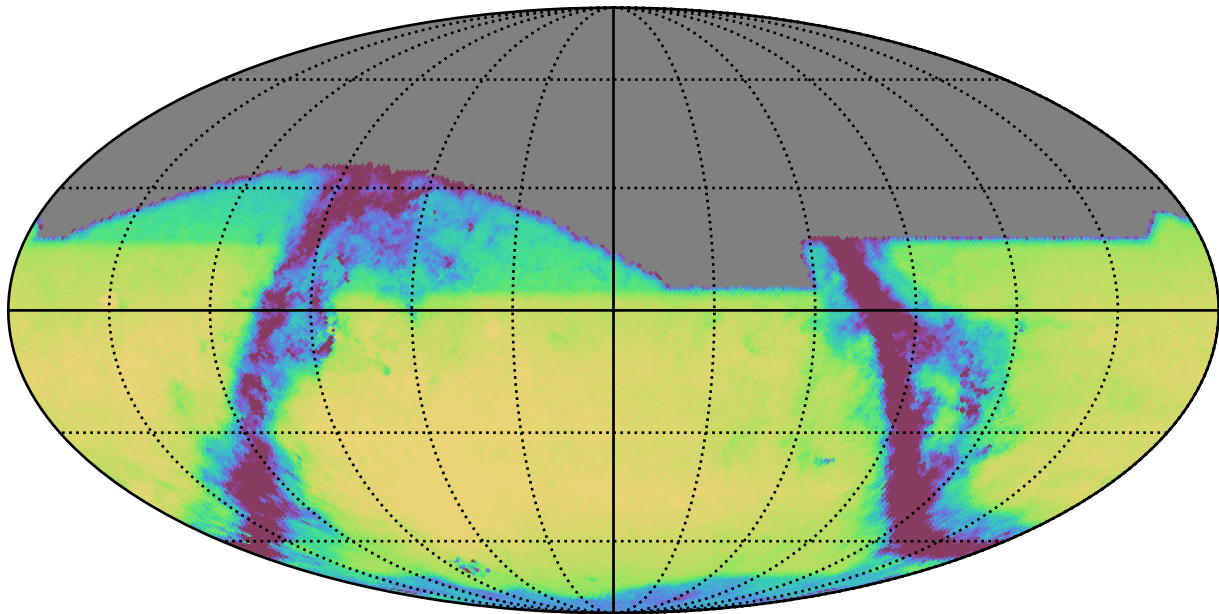
weather_cloudso18v3.4_10yrs All sky r band: Exgal_CoaddM5
