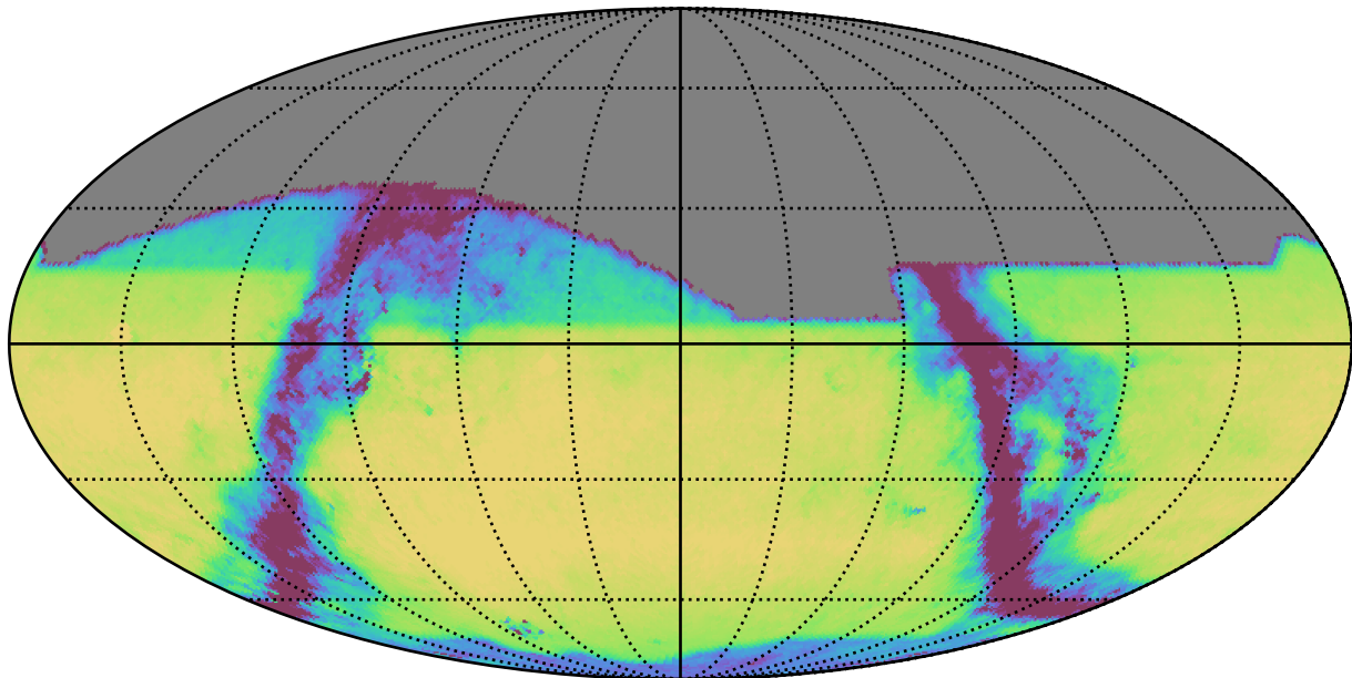
weather_cloudso18v3.4_10yrs All sky i band: Exgal_CoaddM5
