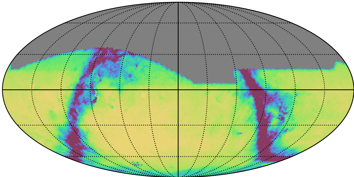
weather_cloudso18v3.4_10yrs All sky g band: Exgal_CoaddM5
