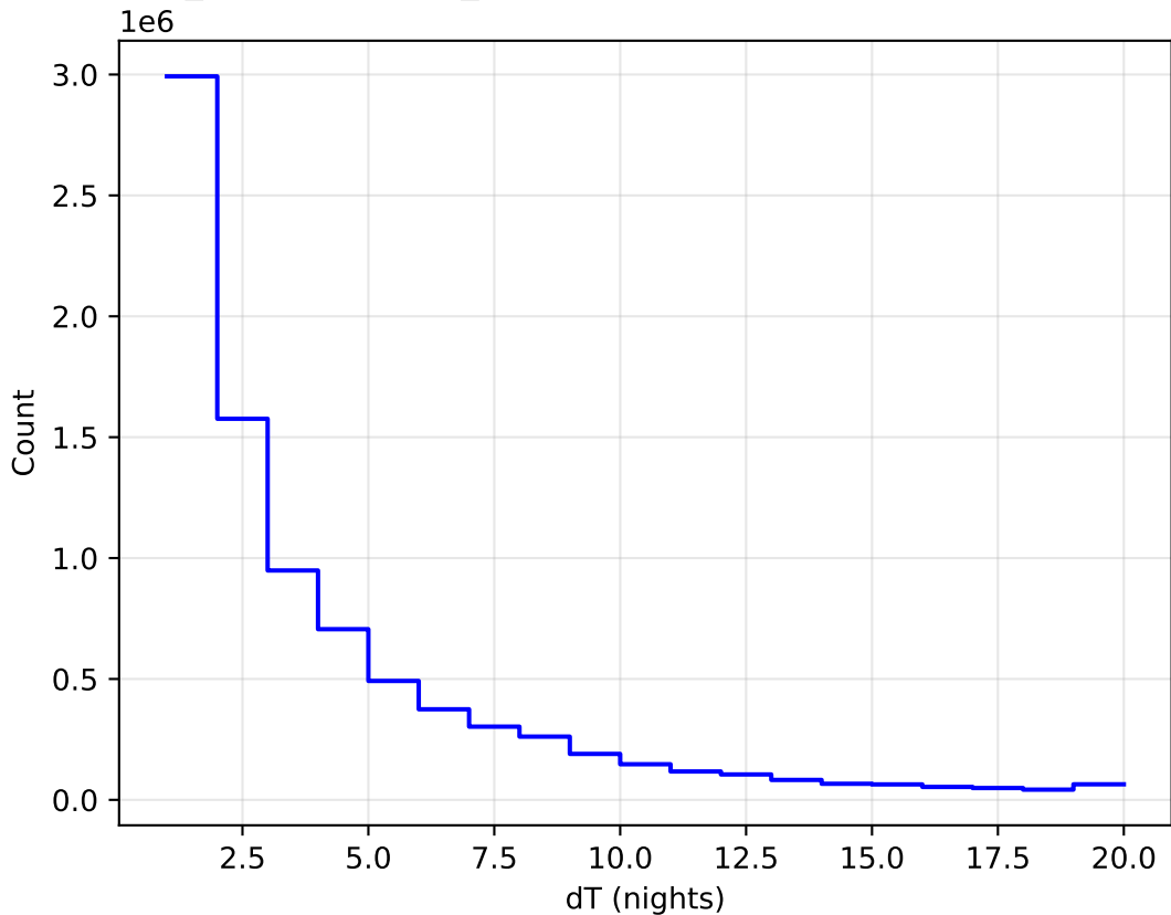
weather_cloudso18v3.4_10yrs WFD all bands: DeltaNight Histogram
