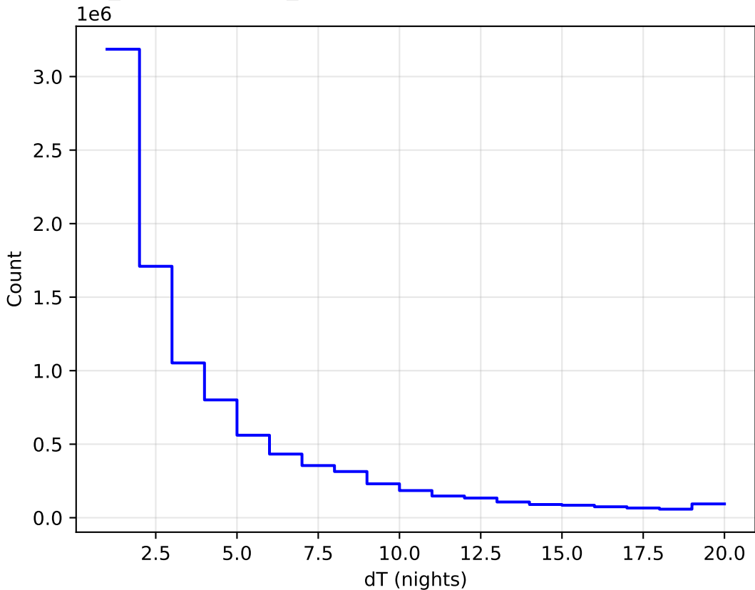
weather_cloudso18v3.4_10yrs All sky all bands: DeltaNight Histogram
