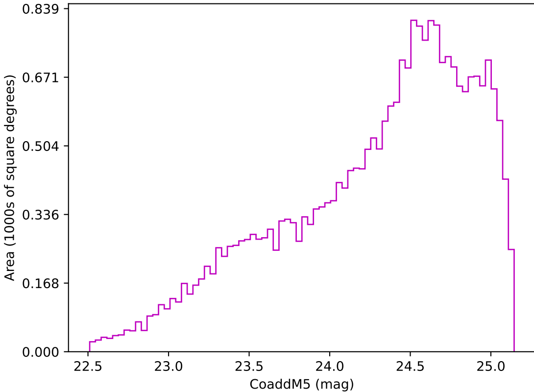
weather_cloudso18v3.4_10yrs Yr 3-4 z band: CoaddM5
