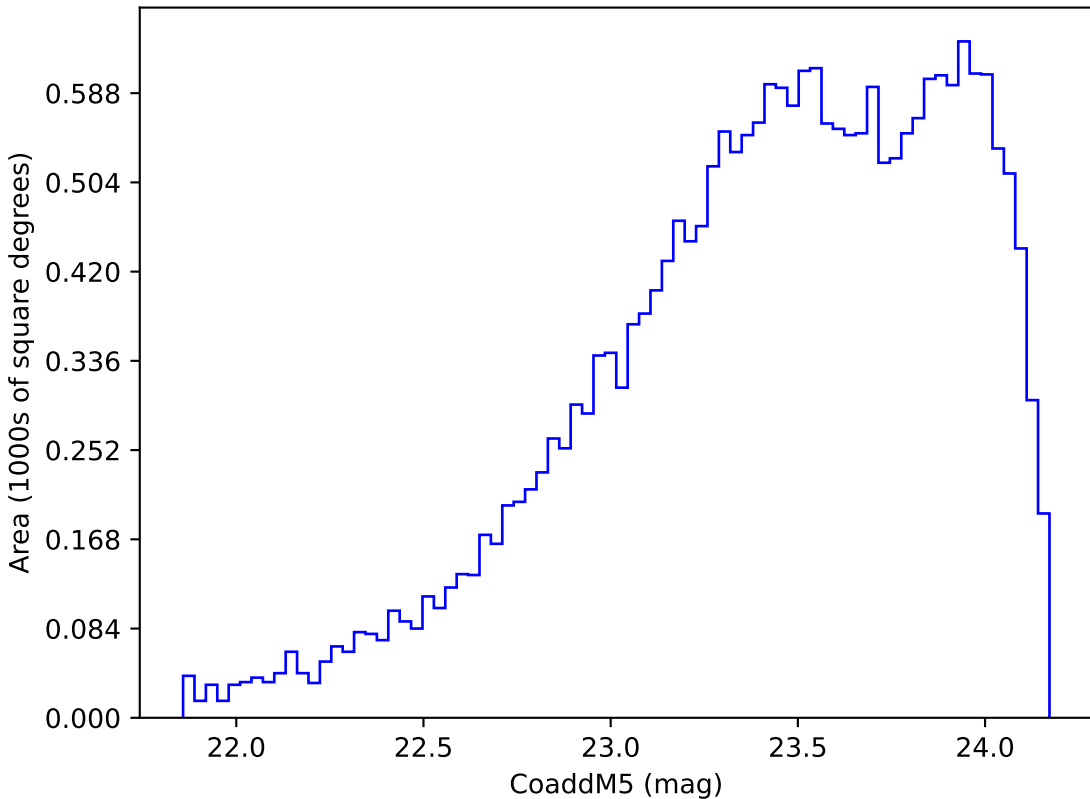
weather_cloudso18v3.4_10yrs Yr 3-4 y band: CoaddM5
