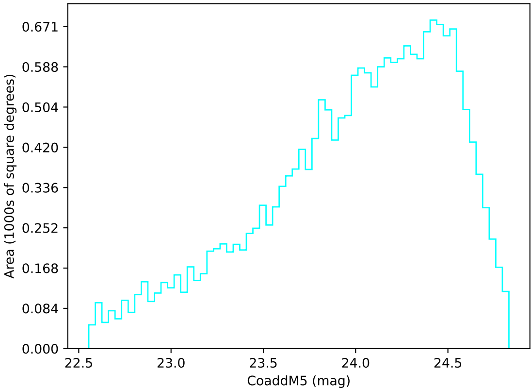
weather_cloudso18v3.4_10yrs Yr 3-4 u band: CoaddM5
