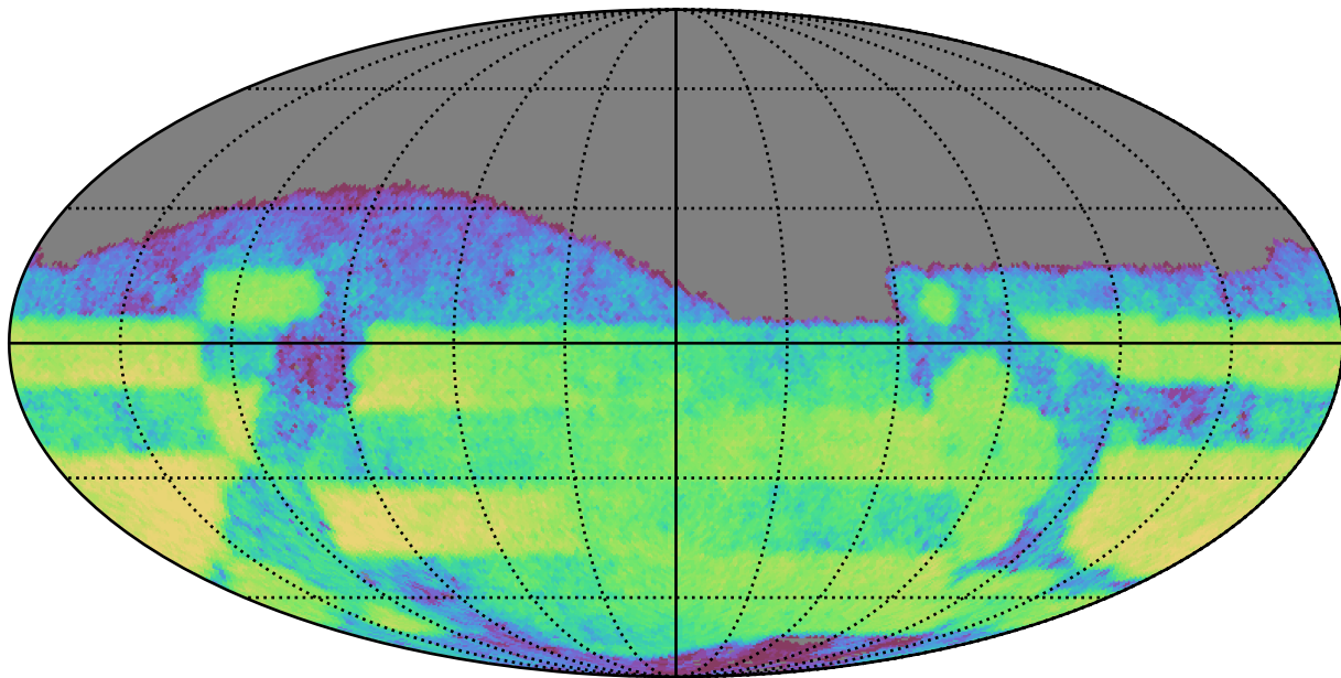
weather_cloudso18v3.4_10yrs Yr 3-4 r band: CoaddM5
