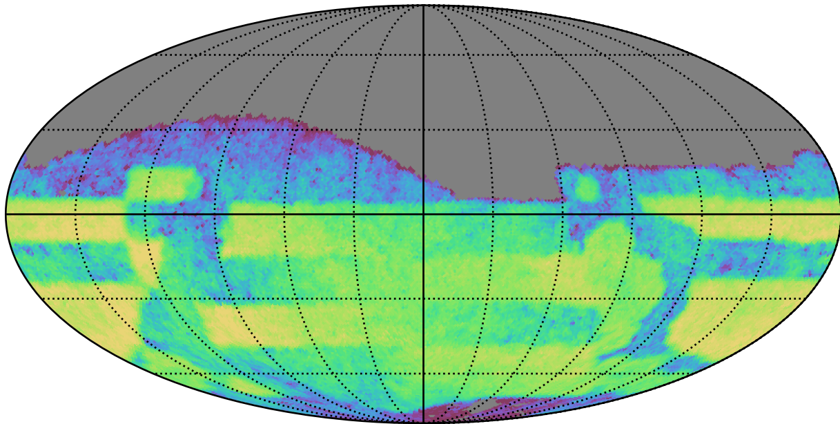
weather_cloudso18v3.4_10yrs Yr 3-4 i band: CoaddM5
