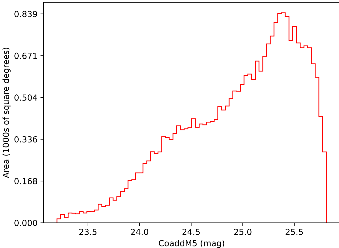
weather_cloudso18v3.4_10yrs Yr 3-4 i band: CoaddM5
