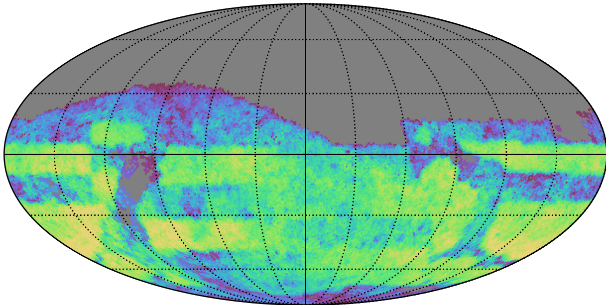
weather_cloudso18v3.4_10yrs Yr 3-4 g band: CoaddM5
