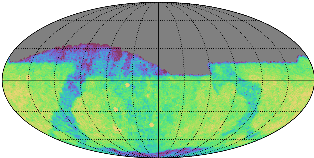
weather_cloudso18v3.4_10yrs Yr 1 z band: CoaddM5
