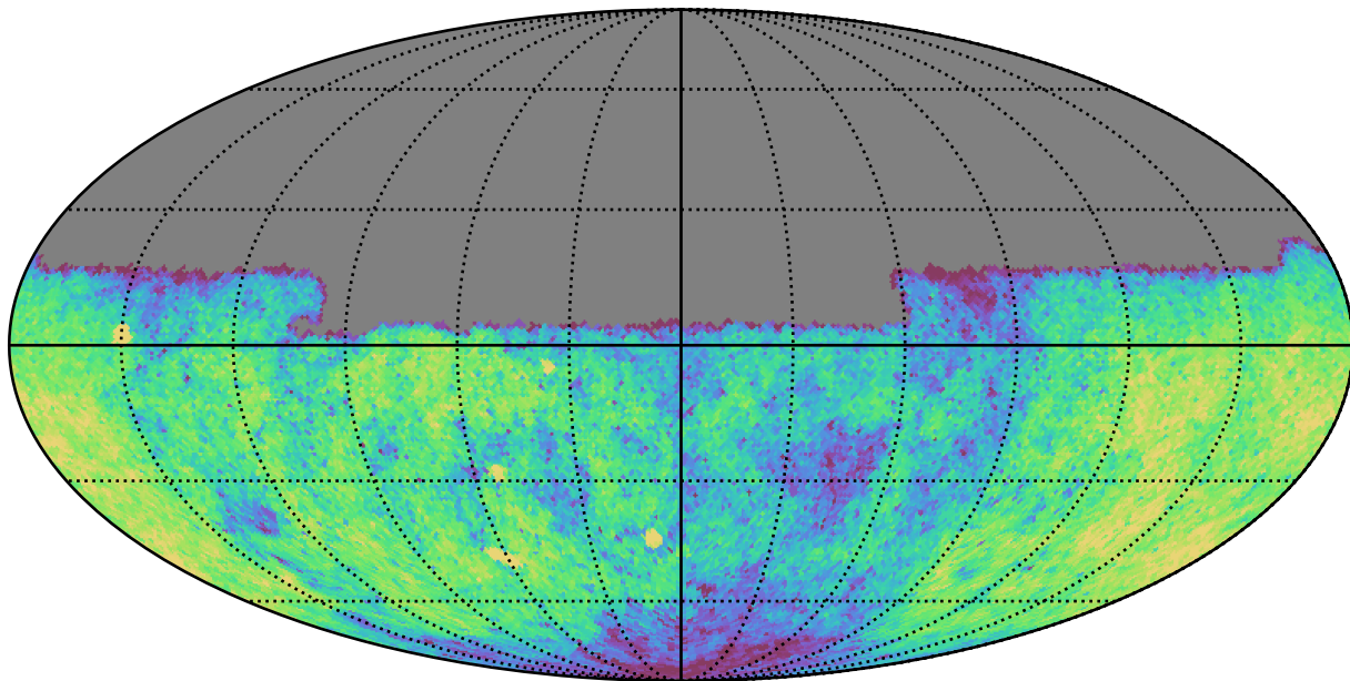
weather_cloudso18v3.4_10yrs Yr 1 u band: CoaddM5
