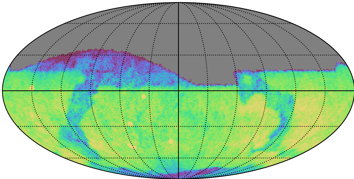
weather_cloudso18v3.4_10yrs Yr 1 r band: CoaddM5
