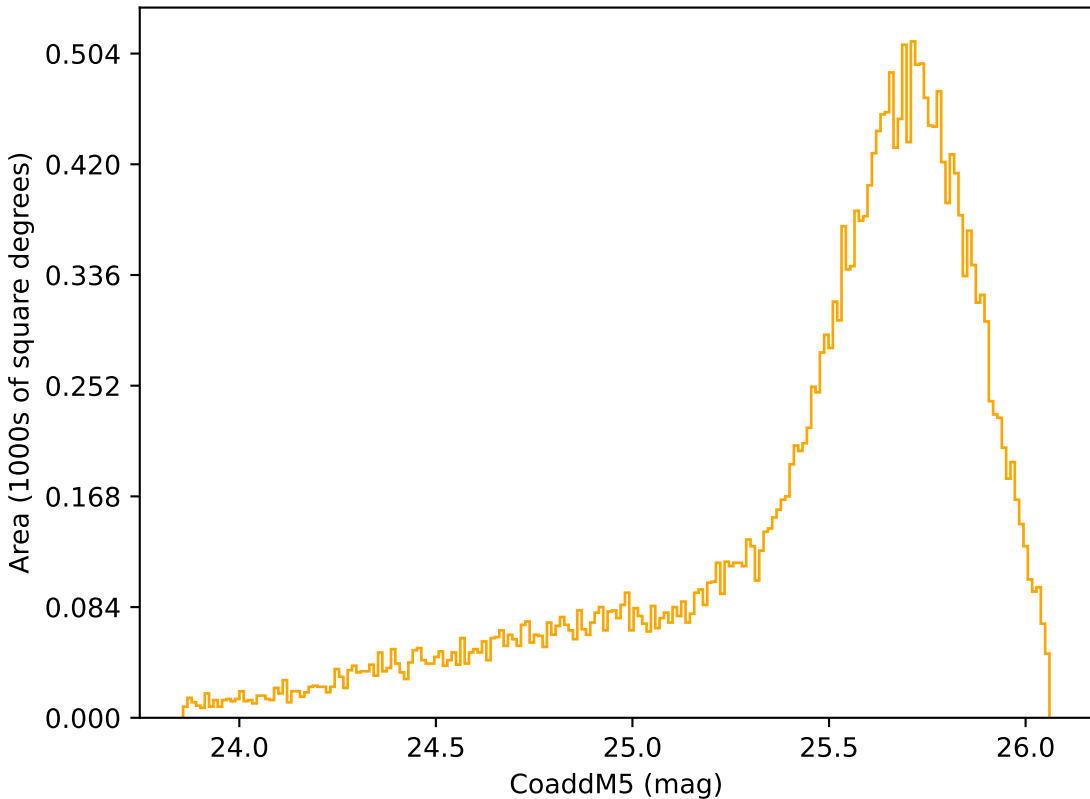
weather_cloudso18v3.4_10yrs Yr 1 r band: CoaddM5
