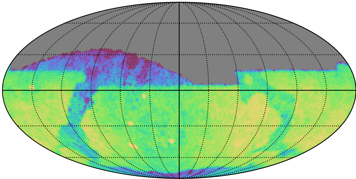
weather_cloudso18v3.4_10yrs Yr 1 i band: CoaddM5
