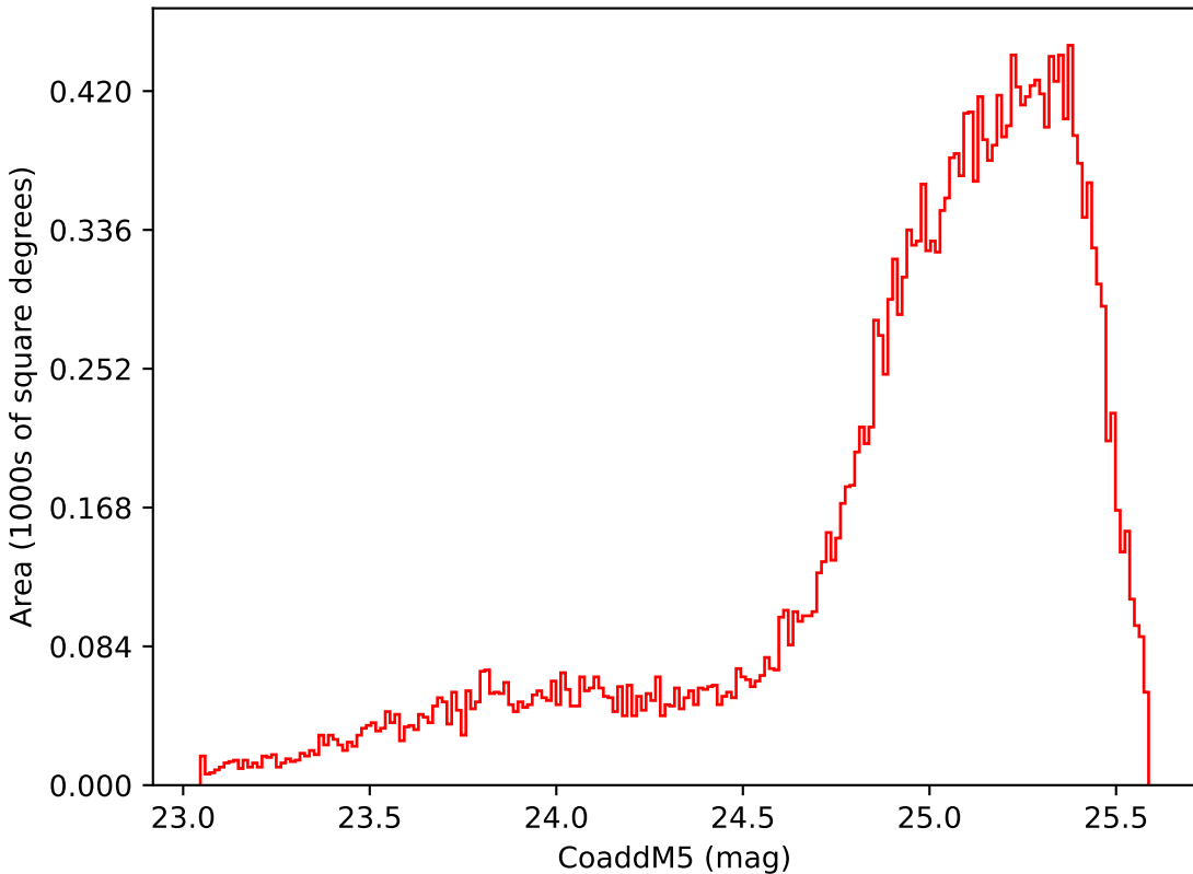
weather_cloudso18v3.4_10yrs Yr 1 i band: CoaddM5
