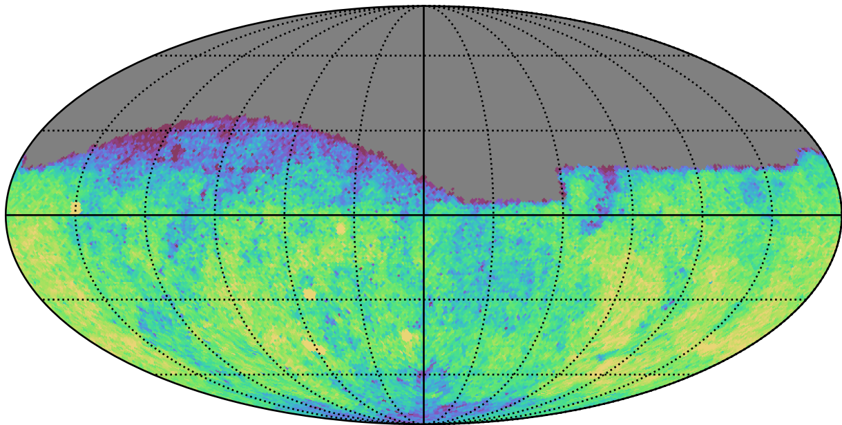
weather_cloudso18v3.4_10yrs Yr 1 g band: CoaddM5
