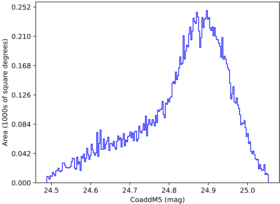
weather_cloudso18v3.4_10yrs WFD y band: CoaddM5
