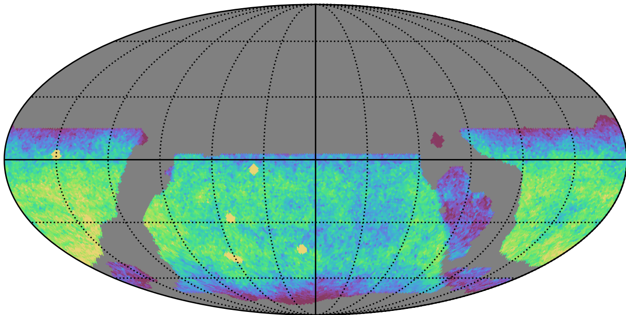
weather_cloudso18v3.4_10yrs WFD u band: CoaddM5
