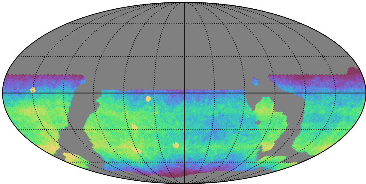
weather_cloudso18v3.4_10yrs WFD r band: CoaddM5
