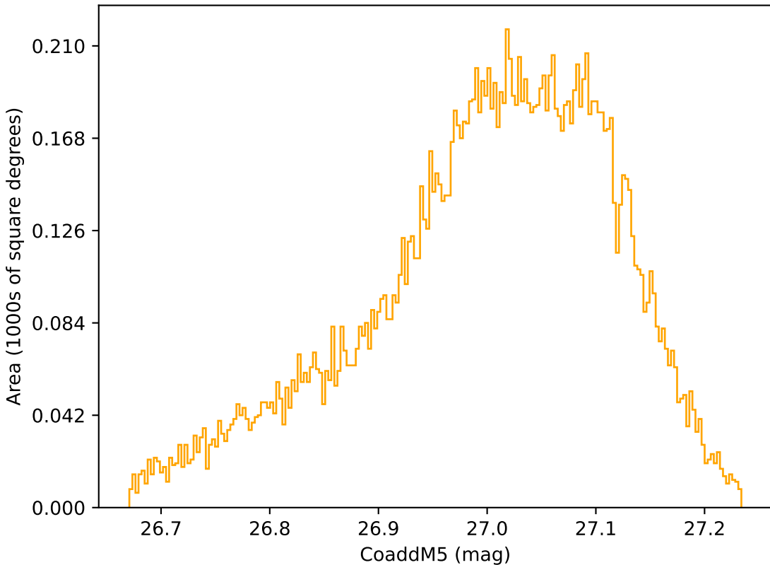
weather_cloudso18v3.4_10yrs WFD r band: CoaddM5
