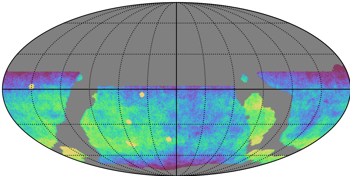
weather_cloudso18v3.4_10yrs WFD g band: CoaddM5
